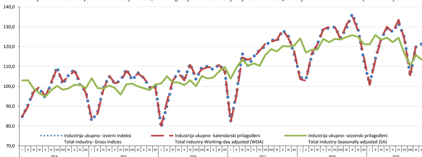
Grafik 1. Vremenska serija industrija ukupno - izvorni, kalendarski i sezonski prilagođeni indeksi: siječanj 2014 - listopad 2019 (2015=100) Graph 1. Time series for total industry - Gross, Working-day and Seasonally Adjusted indices: January 2014 - October 2019 (2015=100)
